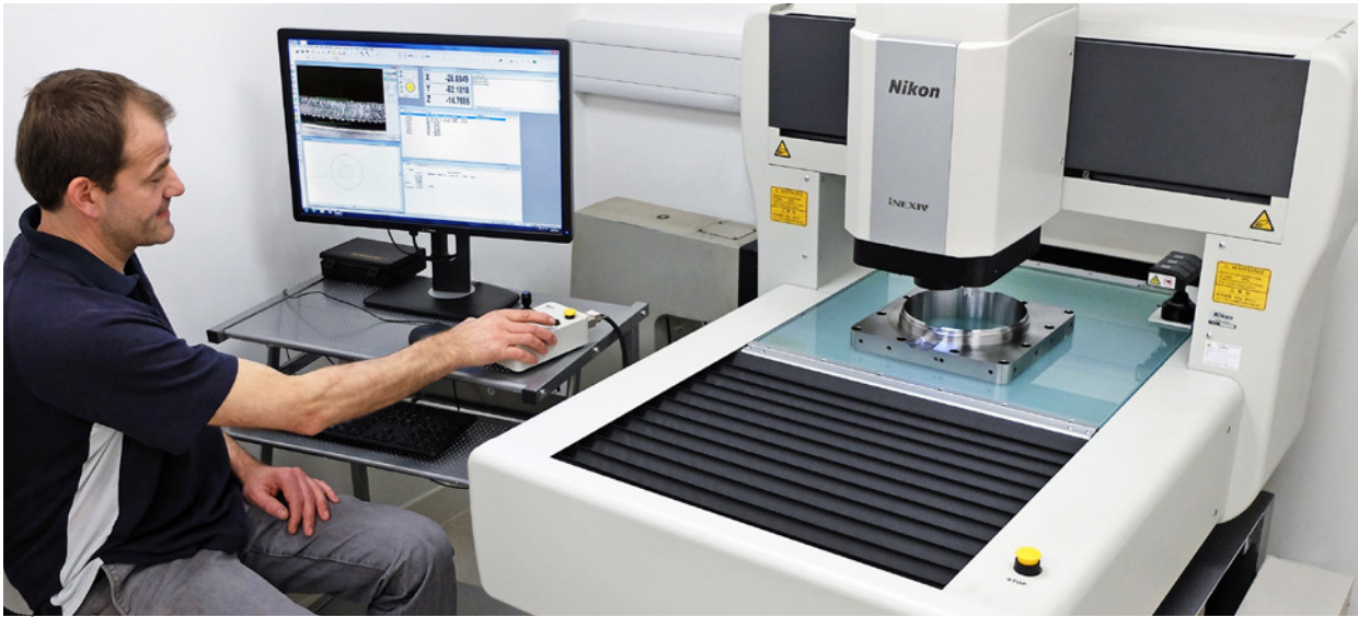
Microtec's managing director, Graham Cranfield inspecting a much larger part on the iNEXIV, in this case a steel mould cavity ring.
